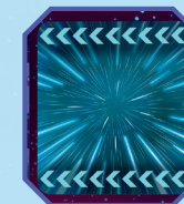
Hyperspace space
