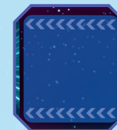
Normal space
